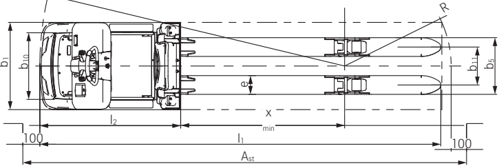
Vista superior OPX 20/25/OPX 20 Plus/OPX 25 Plus
